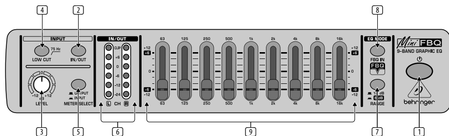
Painel frontal do FBQ800
