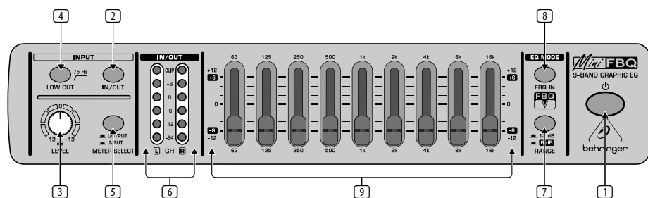
Panel frontal del FBQ800
