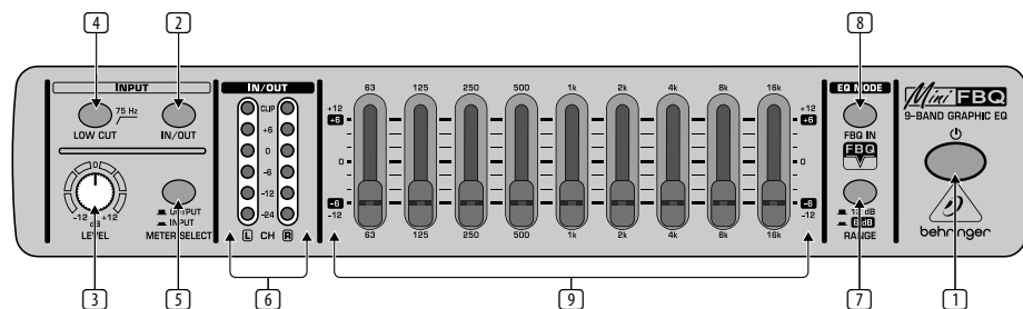
FBQ800 front panel
