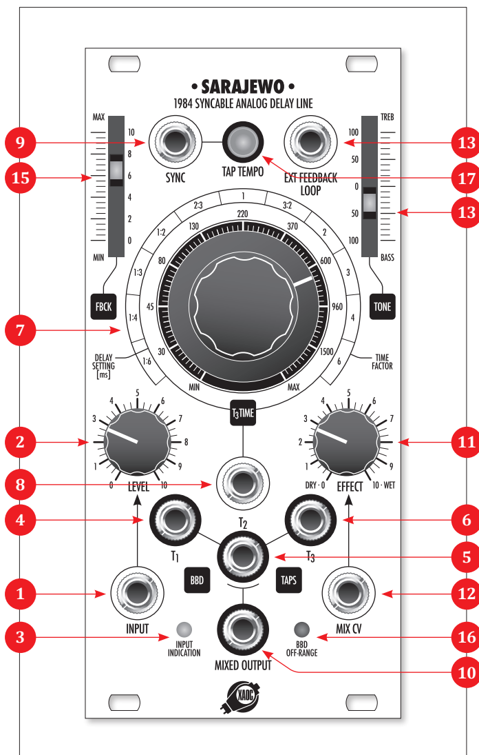
fig. 2: SARAJEWO FRONT PANEL LAYOUT AND CONTROLS
