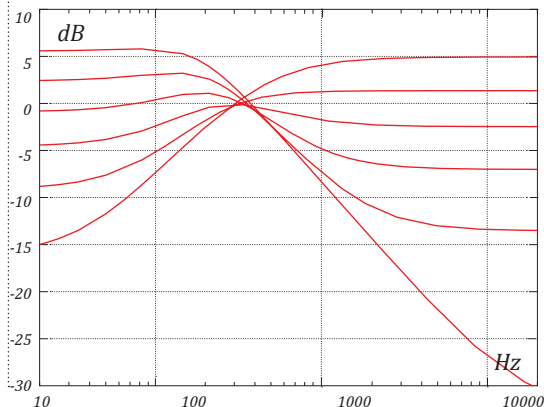
fig. 3: TILT FILTER RESPONSE
