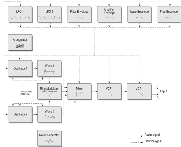
Signal routing
