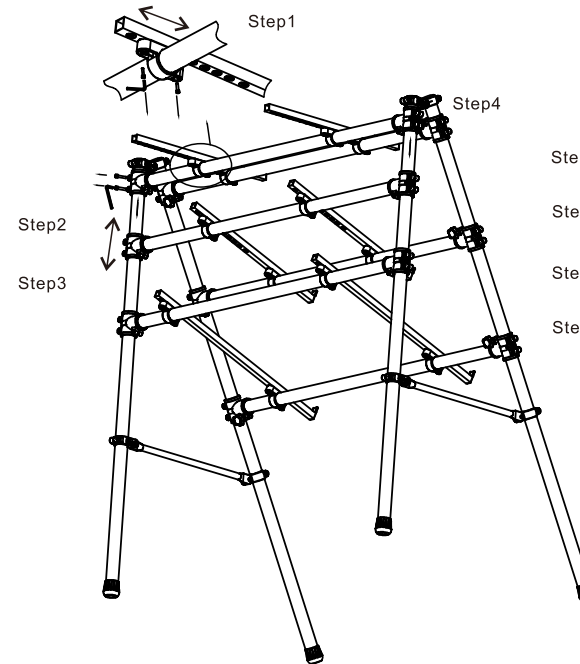
Adjusting stand
