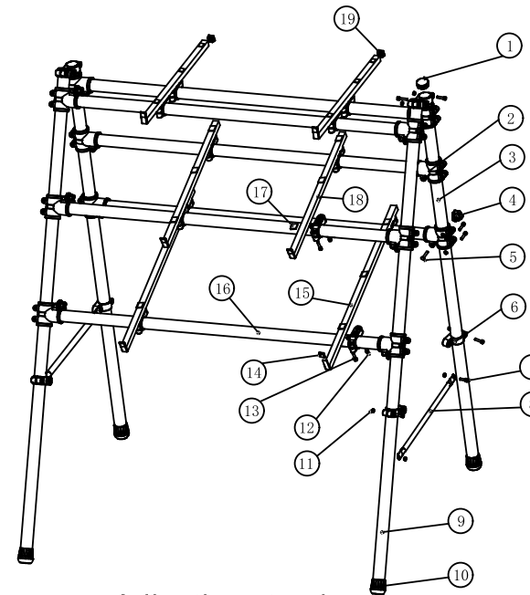
Adjusting stand
